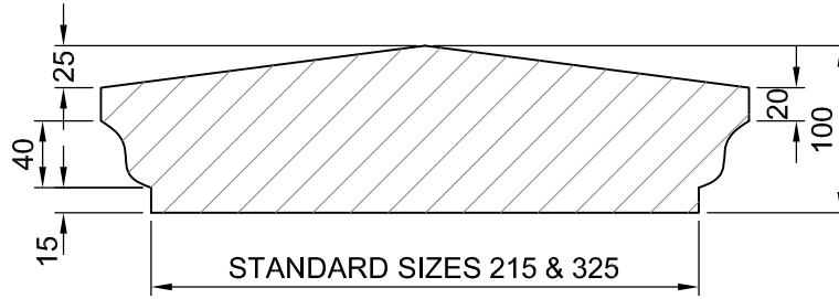
TYPICAL SECTION
